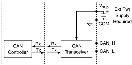
Figure 3. NI 9881 Hardware Overview
